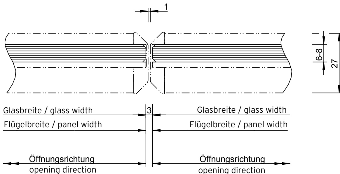
Detail 25-11-12
