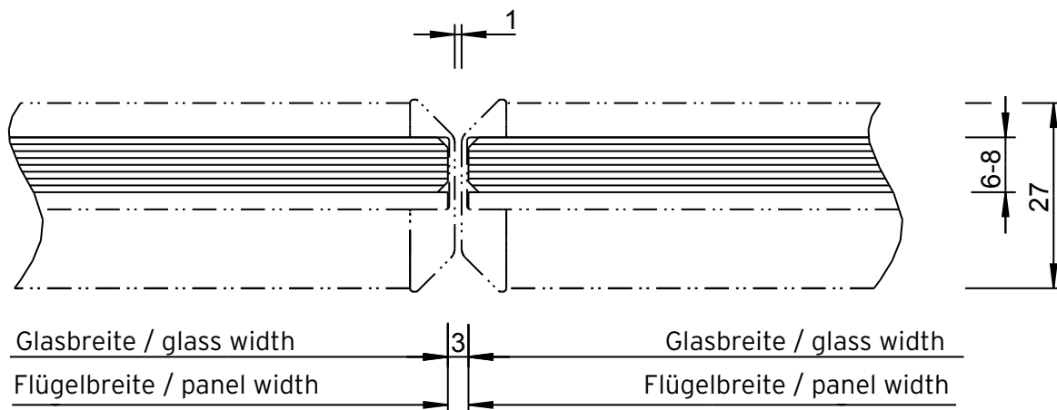
Detail 25-11-0
