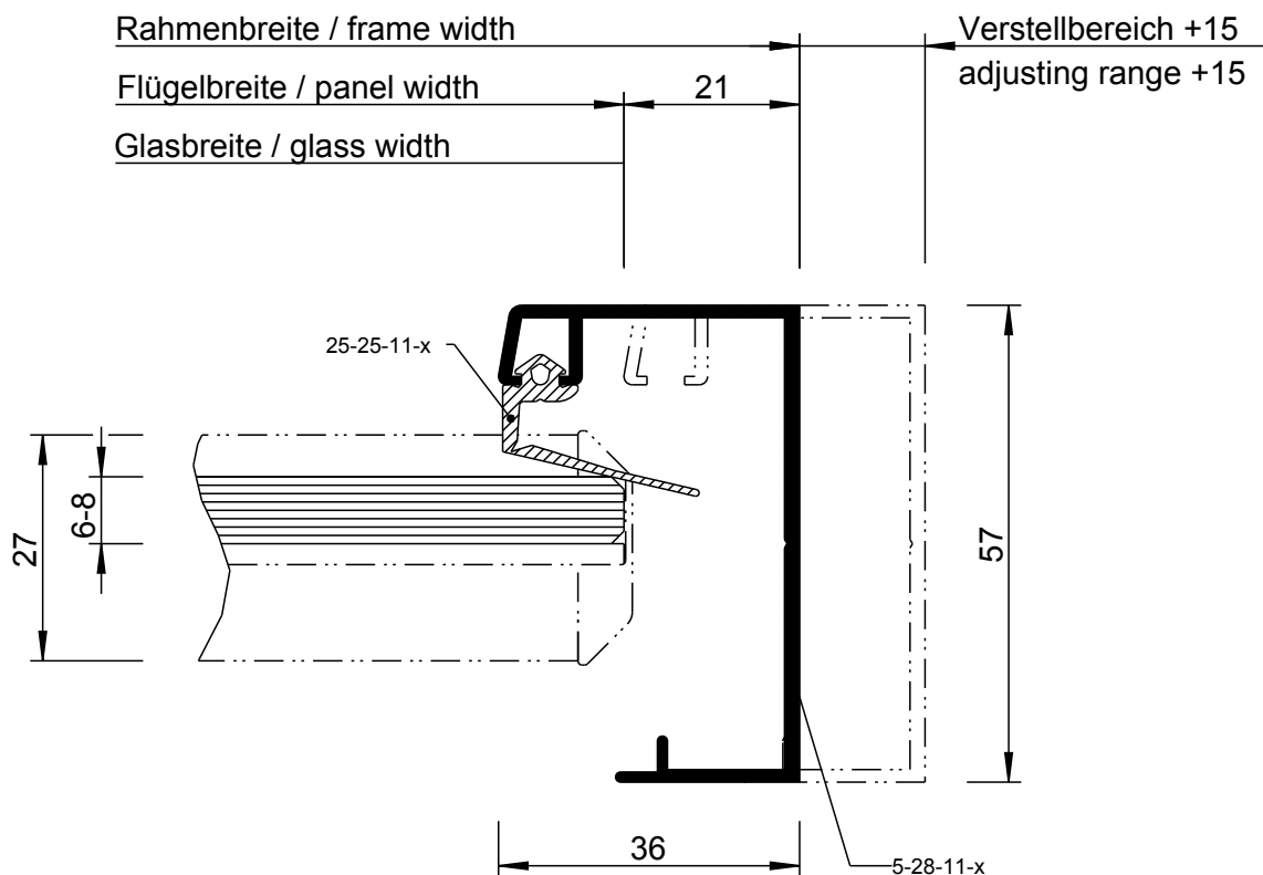
Detail 25-3-5
