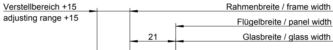
Detail 25-3-6
