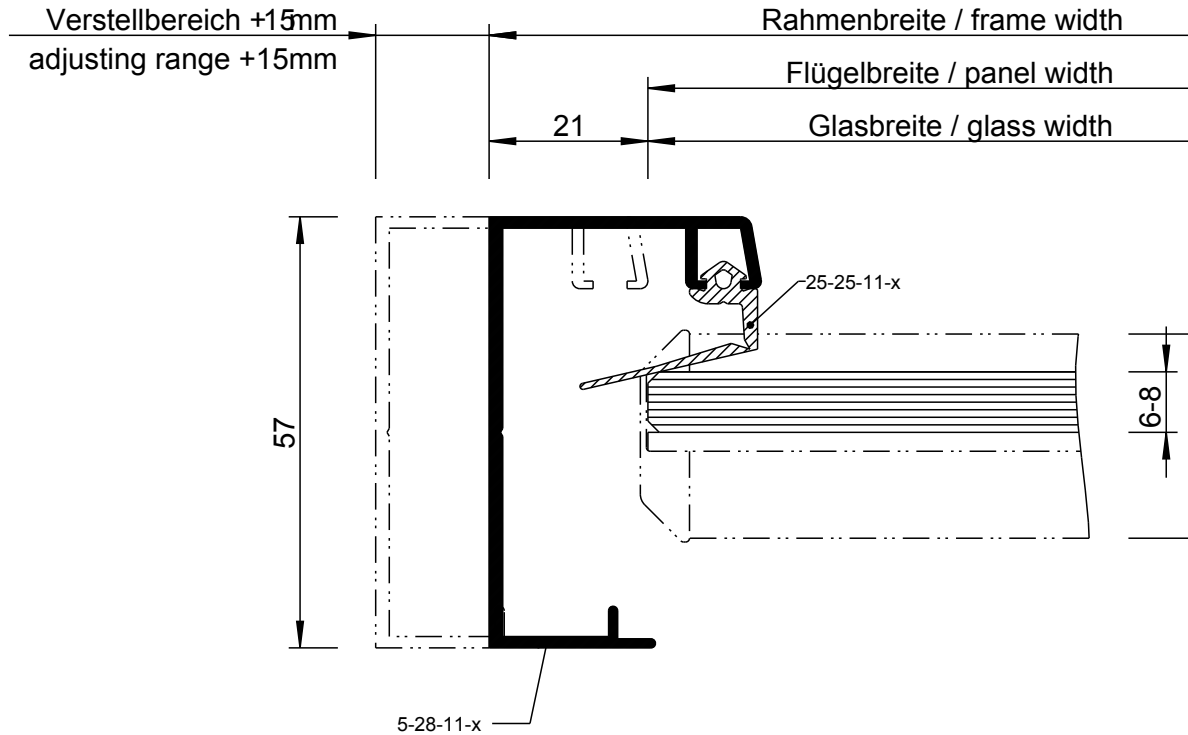
Detail 25-6-3
