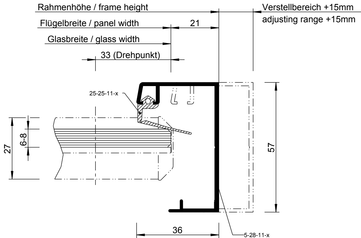
Detail 25-3-3
