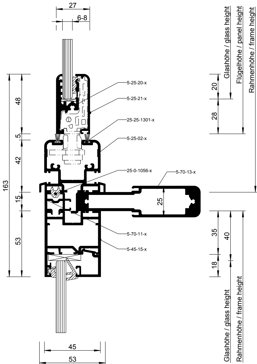
Detail 25-37-2
